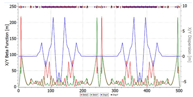
Fig. 2 (Color online) “Resonant” NICA magneto-optical adapted lattice with increased transition energy and missing magnet
